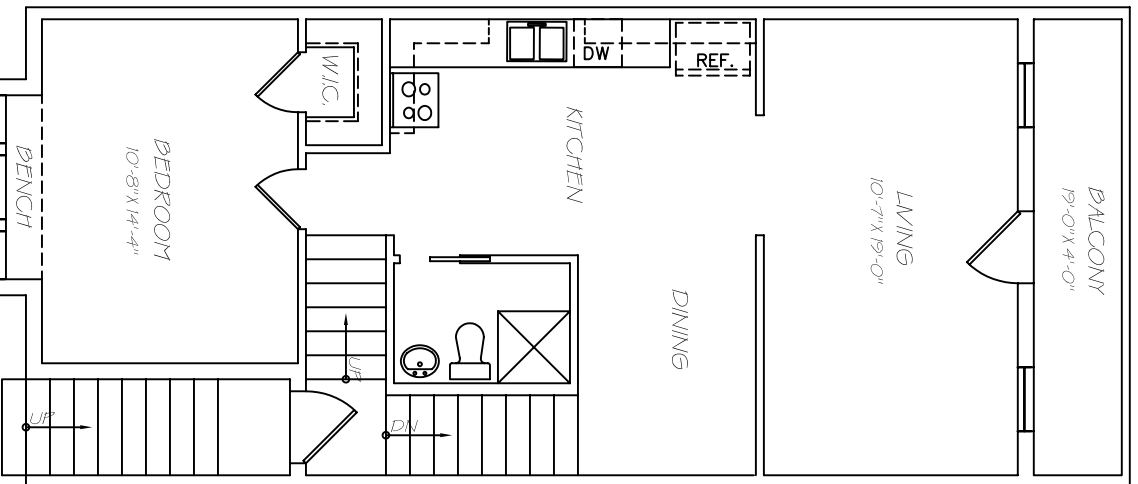
SECOND FLOOR
